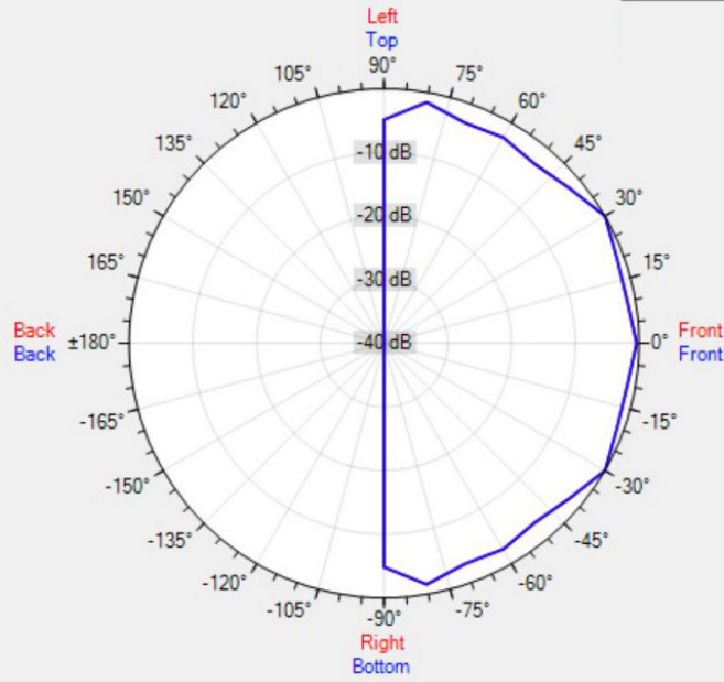
Data Shown: CM4 (Apart Audio) Display Parameters: Frequency: 2000Hz (1/24th Octave)
