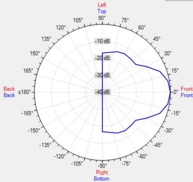
Data Shown: CM4 (Apart Audio) Display Parameters: Frequency: 8000Hz (1/24th Octave)
