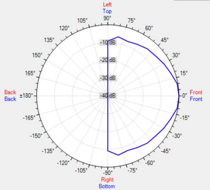
Data Shown: CM6QFT (Apart Audio) Display Parameters: Frequency: 2000Hz (1/24th Octave)
