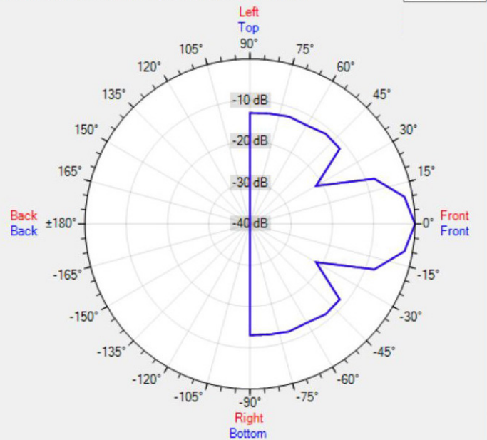
Data Shown: CM6TSMF (Apart Audio) Display Parameters: Frequency: 8000Hz (1/24th Octave)
