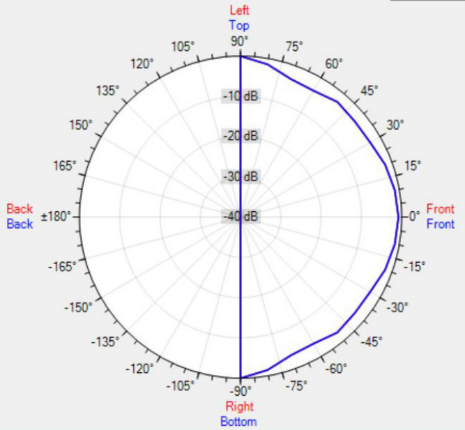
Data Shown: CM6TSMF (Apart Audio) Display Parameters: Frequency: 1000Hz (1/24th Octave)
