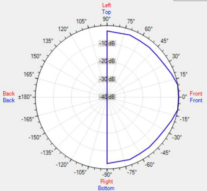
Data Shown: CM6TSMF (Apart Audio) Display Parameters: Frequency: 4000Hz (1/24th Octave)
