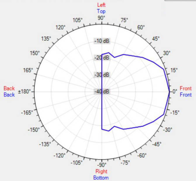
Data Shown: EN-SM6T10-W (APart Audio) Display Parameters: Frequency: 8000Hz (1/24th Octave)
