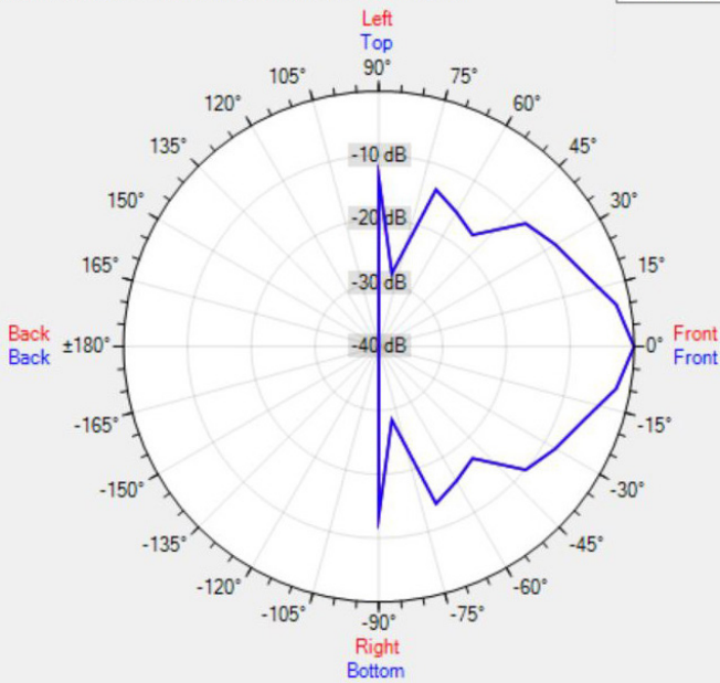
Data Shown: EN-SM6T10-W (APart Audio) Display Parameters: Frequency: 4000Hz (1/24th Octave)
