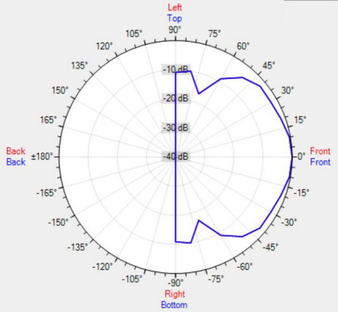
Data Shown: EN-SM6T10-W (APart Audio) Display Parameters: Frequency: 2000Hz (1/24th Octave)
