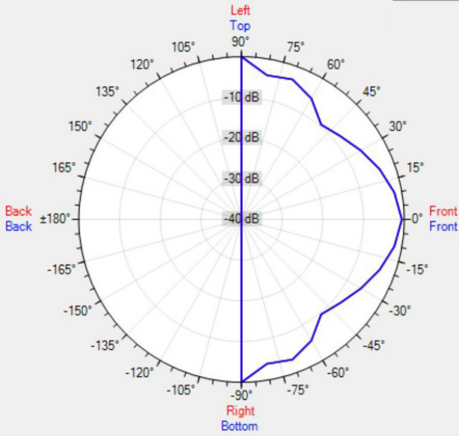
Data Shown: EN-SM6T10-W (APart Audio) Display Parameters: Frequency: 1000Hz (1/24th Octave)
