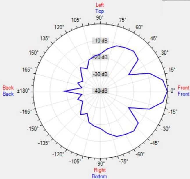
Data Shown: EN-SPH6T20-W (APart Audio) Display Parameters: Frequency: 4000Hz (1/24th Octave)
