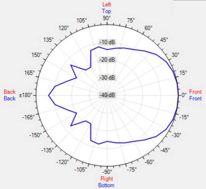
Data Shown: EN-SPH6T20-W (APart Audio) Display Parameters: Frequency: 2000Hz (1/24th Octave)
