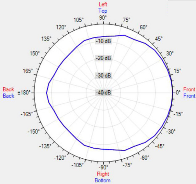
Data Shown: EN-SPH6T20-W (APart Audio) Display Parameters: Frequency: 1000Hz (1/24th Octave)
