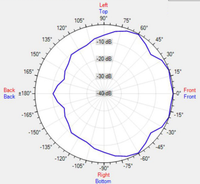
Data Shown: EN-SPH6T20-W (APart Audio) Display Parameters: Frequency: 8000Hz (1/24th Octave)
