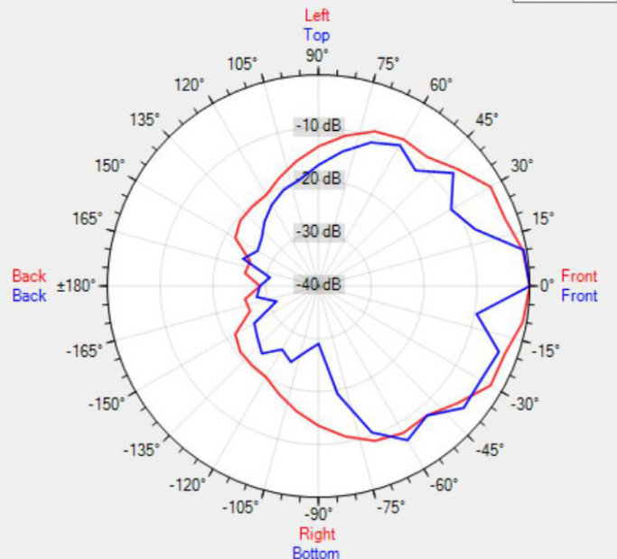
Data Shown: OVO8 (Apart Audio) Display Parameters: Frequency: 8000Hz (1/24th Octave)
