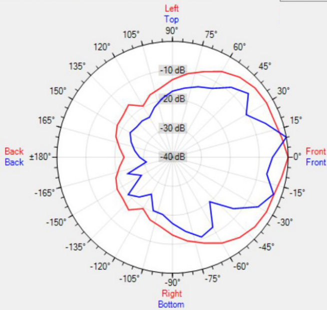
Data Shown: OVO8 (Apart Audio) Display Parameters: Frequency: 4000Hz (1/24th Octave)
