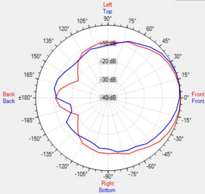
Data Shown: OVO8 (Apart Audio) Display Parameters: Frequency: 1000Hz (1/24th Octave)
