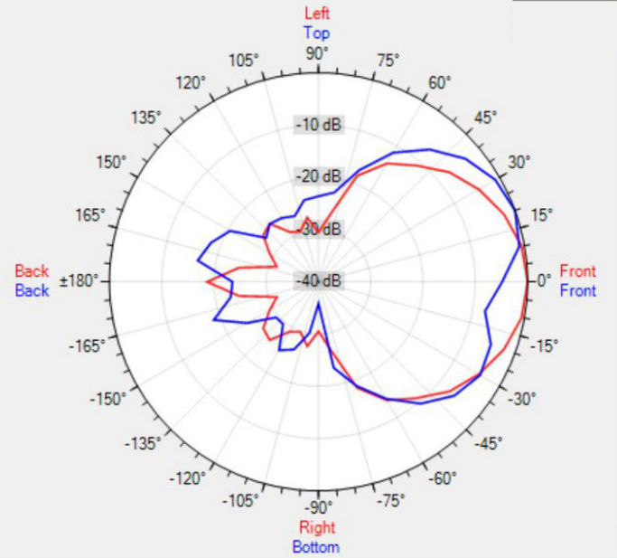
Data Shown: OVO8 (Apart Audio) Display Parameters: Frequency: 2000Hz (1/24th Octave)
