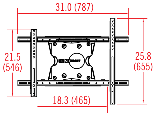
Universal adapter dimensions
