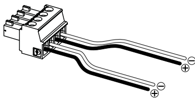
FIG. 2: AUX SEL. IN and PWS OUT connector and wirings.
