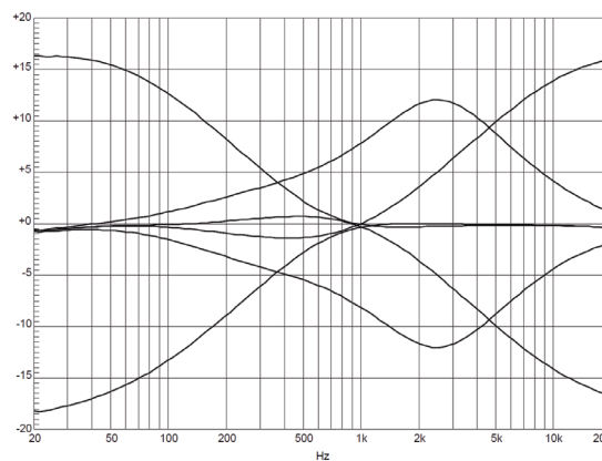
Illustration 2-4: LO/MID/HI filters
