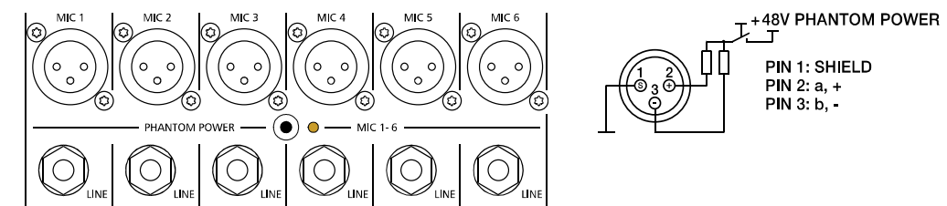
Illustration 2-1: Microphone input
