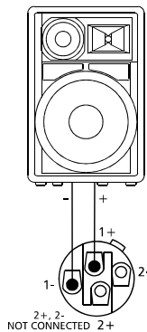
Illustration 2-11: Connection of a passive speaker
