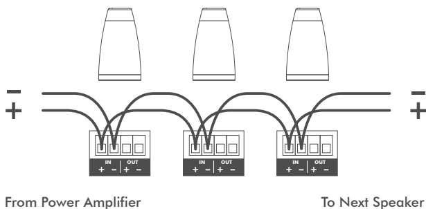
FIGURE 17: PARALLEL CONNECTION
